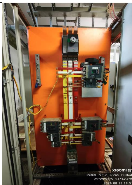
4. QDG 05 2300x1200x800 porta dupla
