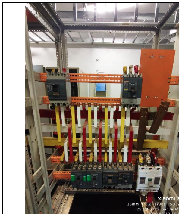
1. QDG 02 2300x1200x800 porta dupla
